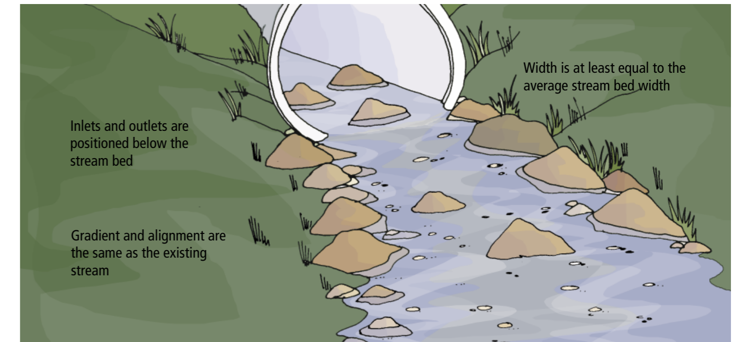
A "low slope" culvert
