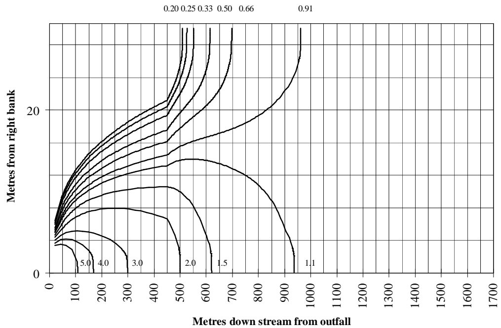
Figure 5e: Predicted dye concentrations at a flow of 6.5 \text{ m}^3/\text{s} for site B. K_q values from Table 3. Values expressed as the ratio of predicted /fully-mixed concentrations.
